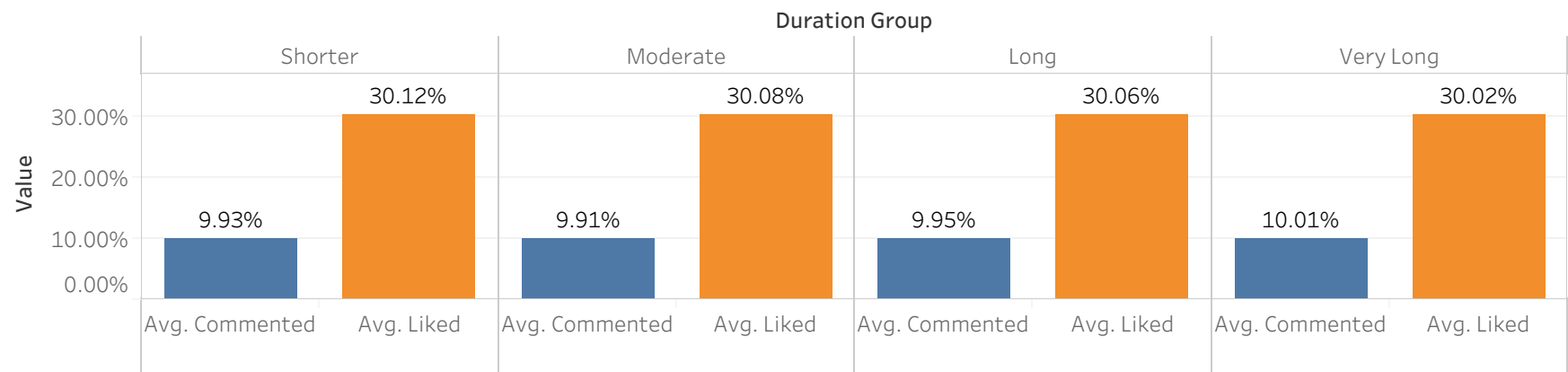
Like vs Comment Rate by Video Length
