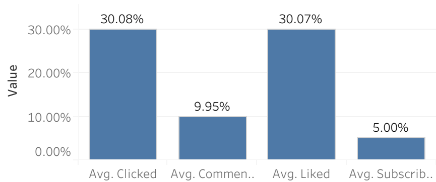
Overall Engagement Rates
